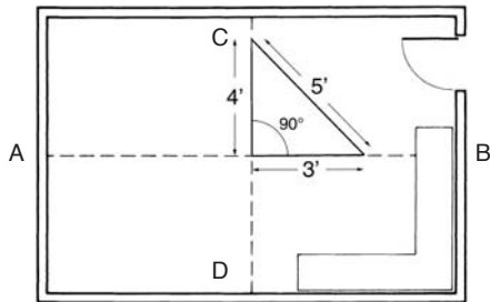
Fig. 6 - Square layout.
